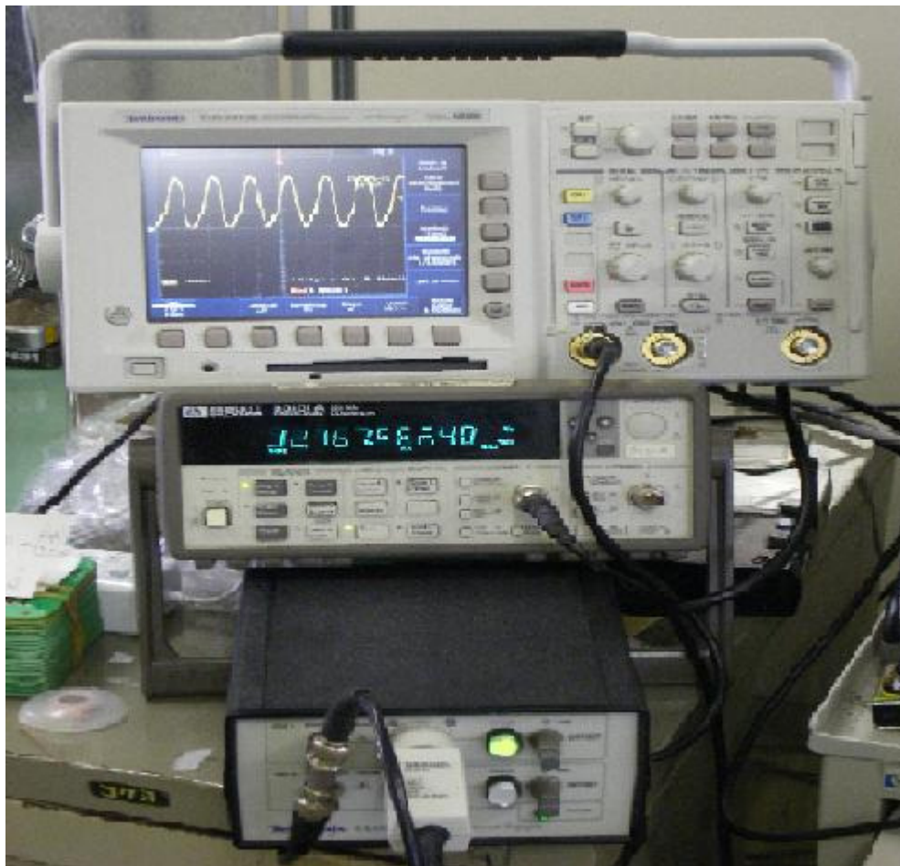
Test set-up for quartz circuit matching service
